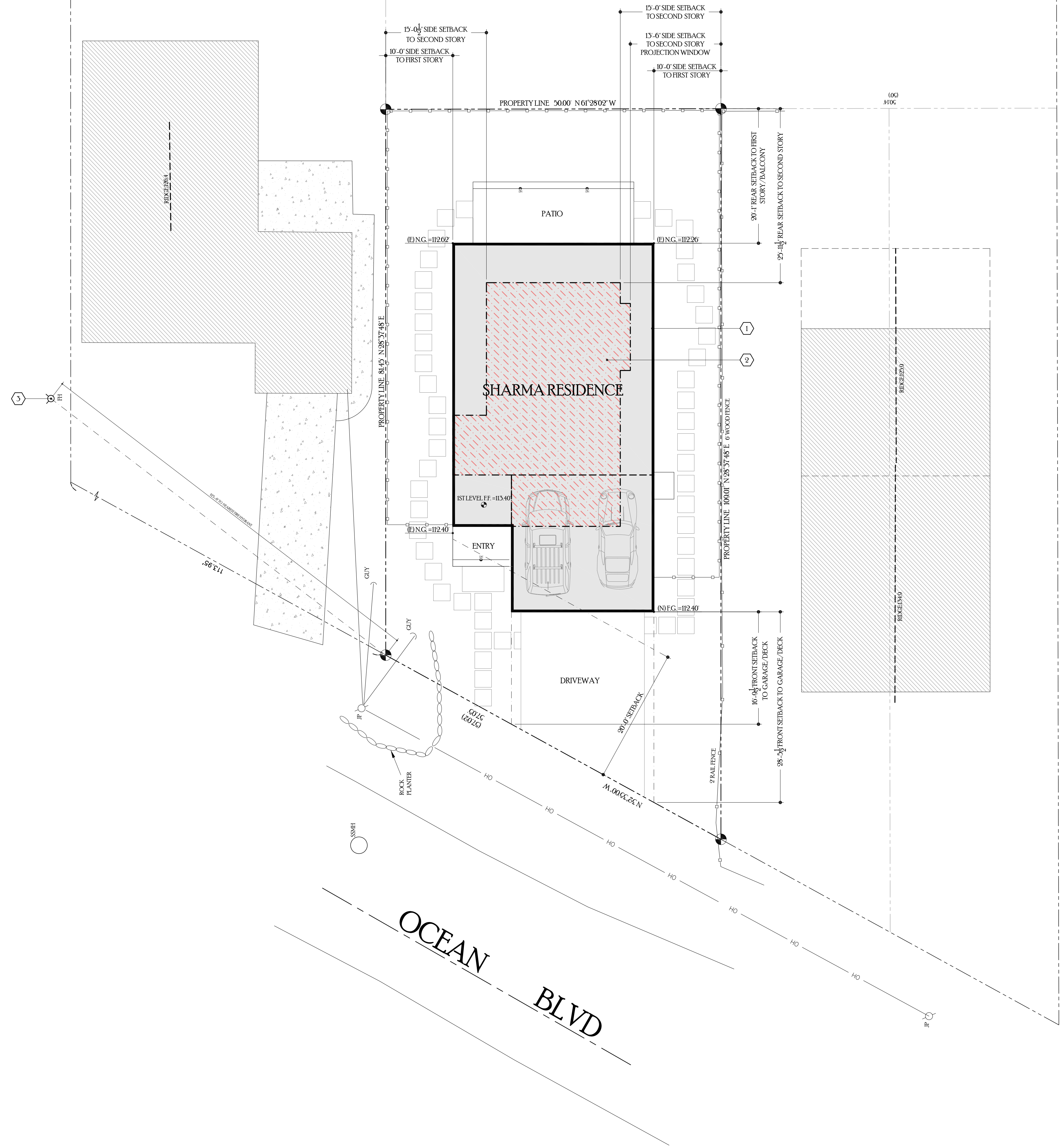
SITE PLAN
